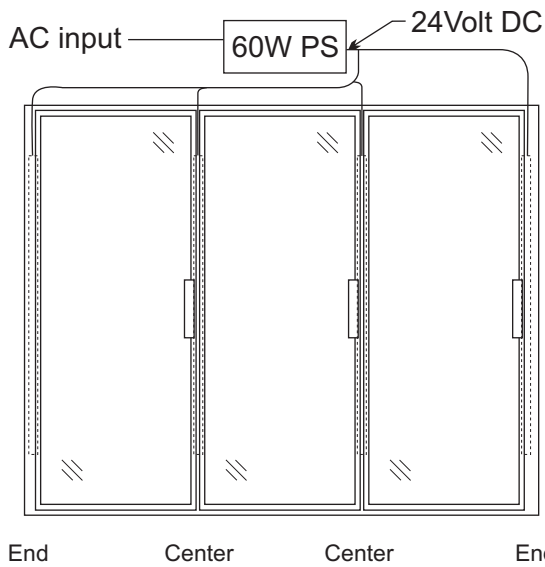
3 Door Case = Two End Units & Two Center Units
