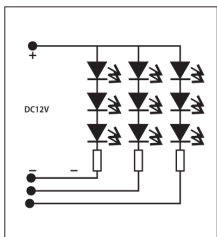
Circuit Diagram:
